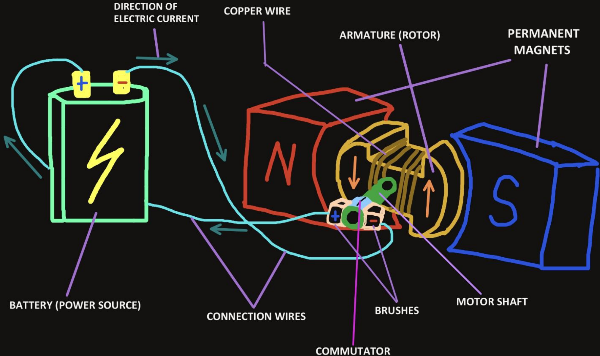
ABOVE: Diagram of a DC Motor that uses permanent magnets to function.
